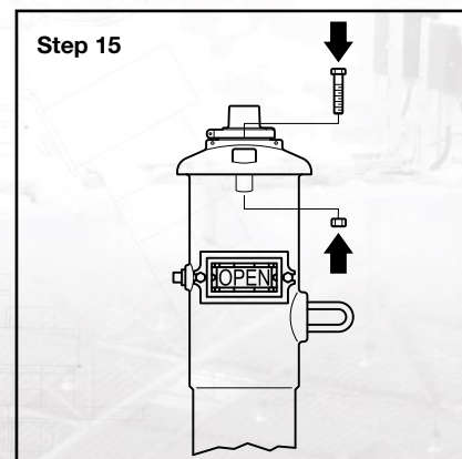
Step 15. Secure the cap to the body with bolts and nuts.
