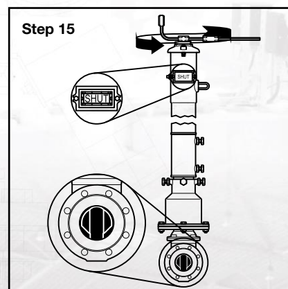
Step 15. Attach the wrench to the operating nut and rotate counter-clockwise. Observe the gate valve waterway to verify the wedge is in the fully SHUT position. Observe the indicator to verify the SHUT targets are centered in the windows.
