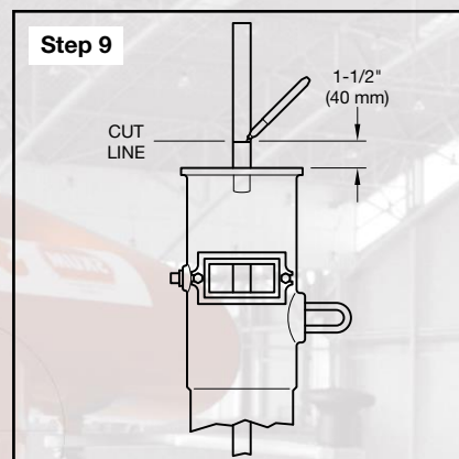
Step 9. Mark a cut line on the connection tube 1 1/2 in. (40 mm) above the top flange of the body.
