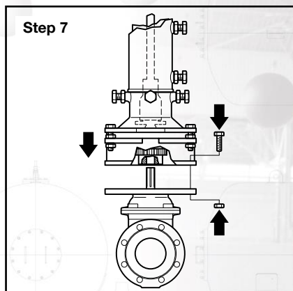
Step 7. Temporarily attach the indicator to the gate valve mounting flange with bolts and nuts. Ensure the connection tube coupling remains engaged onto the reducing gear top cap.
