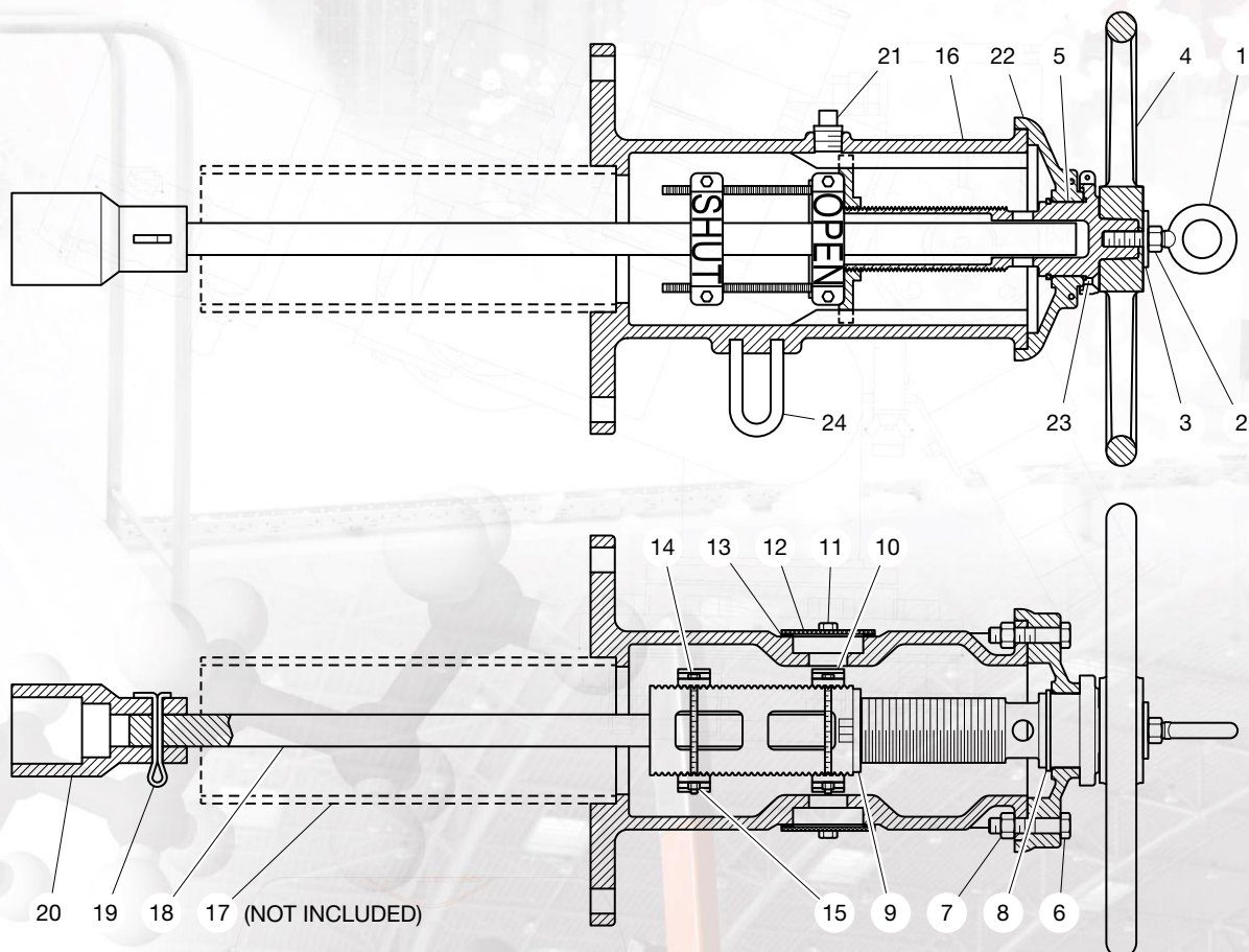
FIGURE 5 CROSS WALL INDICATOR POST ASSEMBLY
