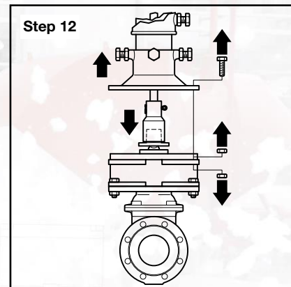
Step 12. Temporarily detach the indicator from the reducing gear, and raise the indicator to gain access to the reducing gear top cap. Engage the connection tube coupling onto the reducing gear top cap.
