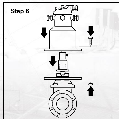
Step 6. Temporarily engage the connection tube coupling onto the gate valve top cap and attach the indicator to the gate valve mounting flange with bolts and nuts.
