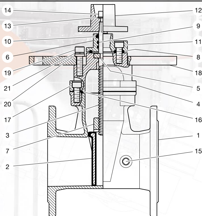
FIGURE 1 POST INDICATOR GATE VALVE ASSEMBLY
