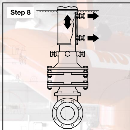
Step 8. Loosen the jam nuts and bolts to free the indicator outer pipe from the inner pipe. Adjust the outer pipe bury line even with finished grade.
