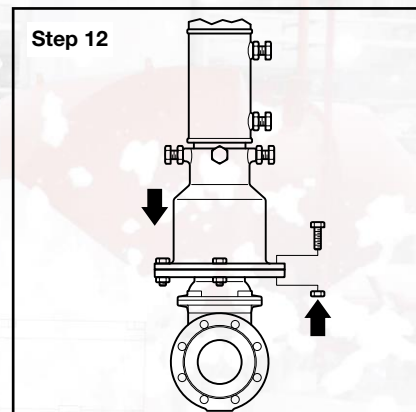
Step 12. Secure the indicator to the gate valve with bolts and nuts.
